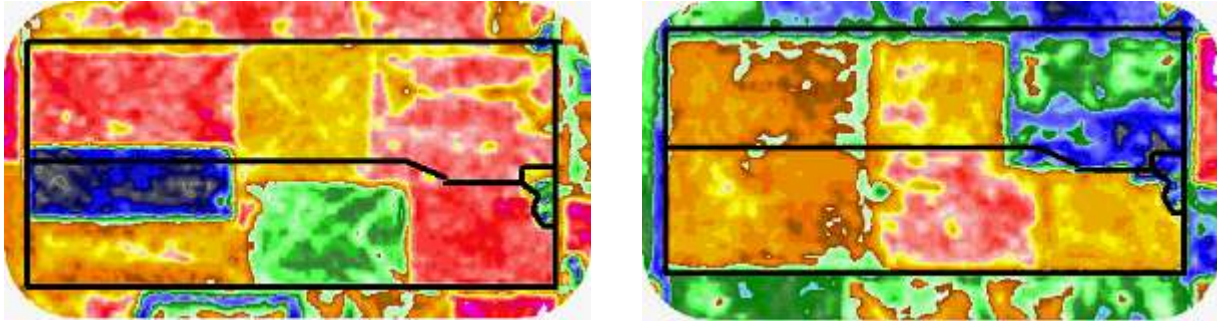
Figure 1. Example of variation in the Normalised Difference Vegetation Index (NDVI) as a result of merging 7 paddocks into two 65 ha paddocks in spring 1991 (left) and the same paddocks in spring 1997 (right).
