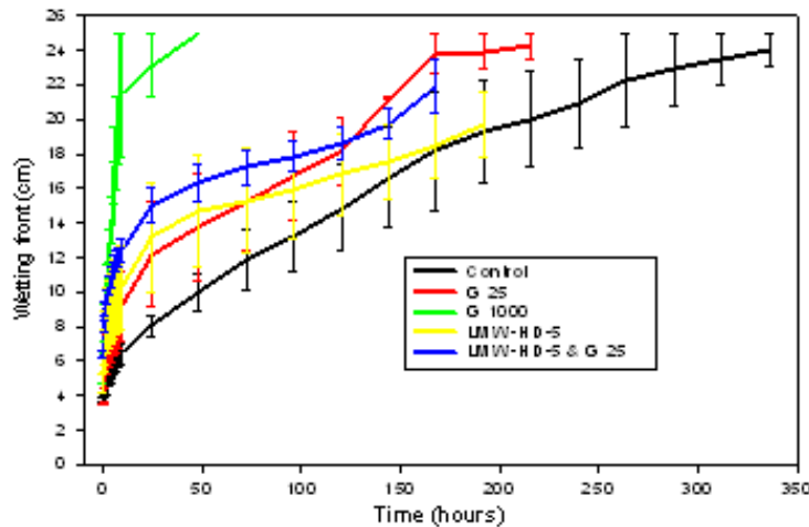
Figure 4. Depth of wetting front against time under different treatments. (G, gypsum; LMW, low molecular weight; HD, high density; numbers represent rate of application in kg ha -1 ).
